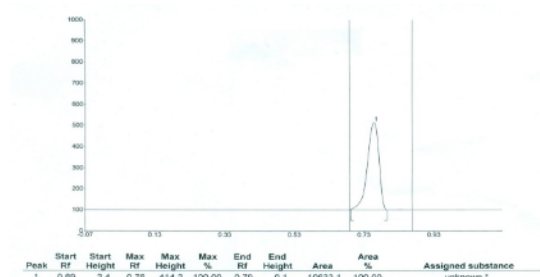
Fig. 2. HPTLC Spectrum of Mangiferin
