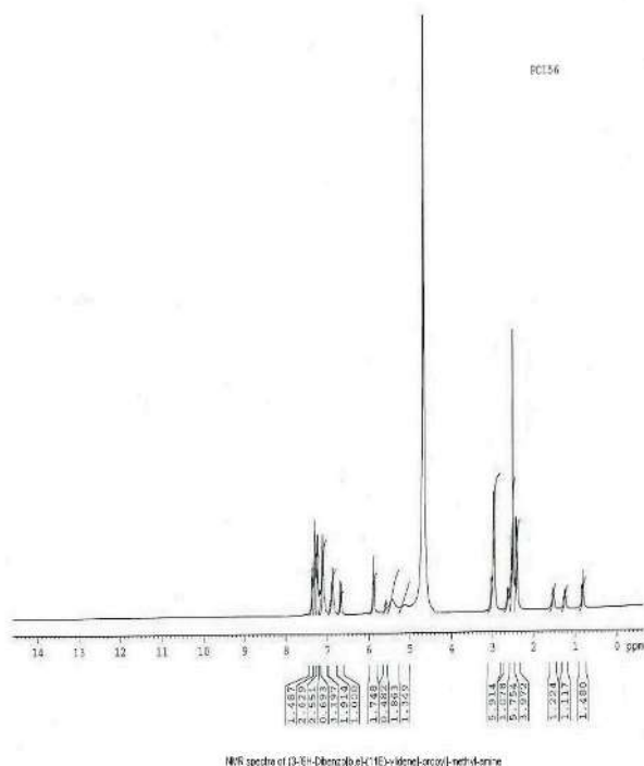
Graph 2: NMR report for the compound PC 156
