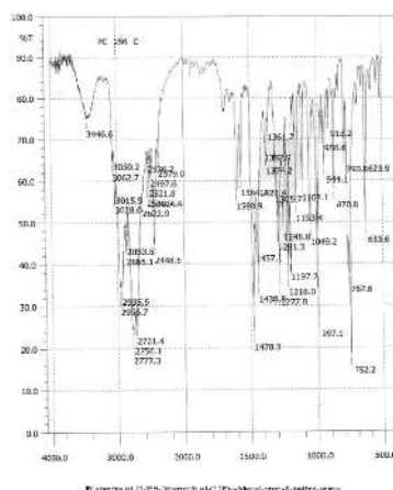
Graph 1: IR report for the compound PC 156
