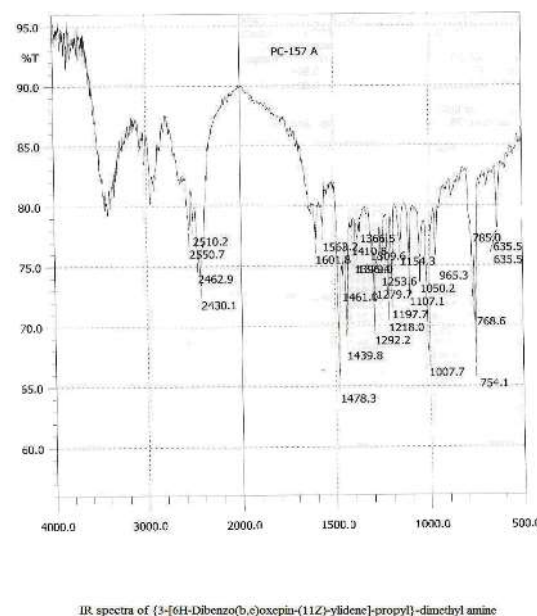
IR spectra of (3-[6H-Dibenzo(b,e)oxepin-(11Z)-ylidene]-propyl)-dimethyl amine
