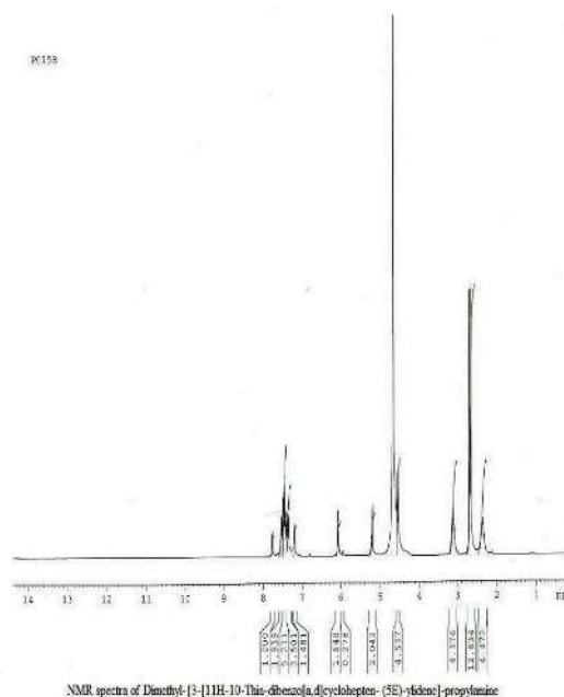
Graph 5: NMR report for the compound PC 158
