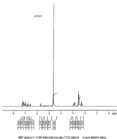
Graph 4: NMR report for the compound PC 157
