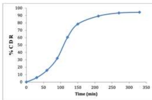
Figure 3: Dissolution Profiles Lornoxicam Floating tablet Batch F12
