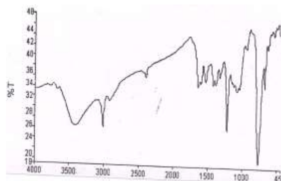
Figure 2: FTIR Spectra of Lornoxicam +Polymer HPMC 50cps(1:1)
