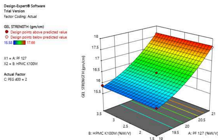
Fig.2 Response surface plot of gel strength
