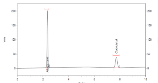
Figure.3: Chromatogram of COB and ATA at 272 nm from Pharmaceutical dosage form (EVOTOZ)
