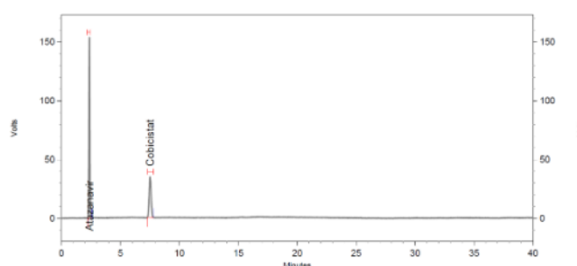
Figure. 6: Forced degradation study at 3 rd day with alkali
