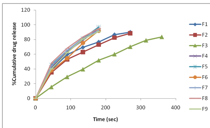
Figure 4: % cumulative drug release of formulations F1 – F9
