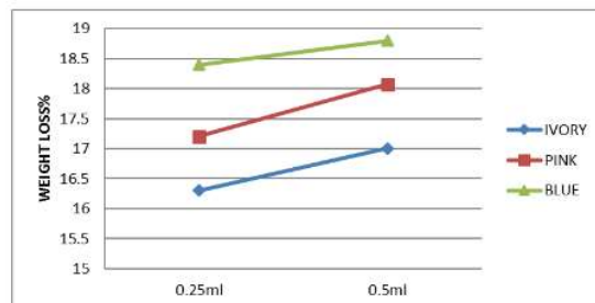
Figure 6: Abrasion resistance of silk fabrics when water based perfume is sprayed in different amount
