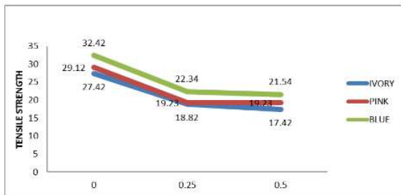
Figure 3: Tensile strength of silk fabrics when ethanol based perfume is sprayed in different amount
