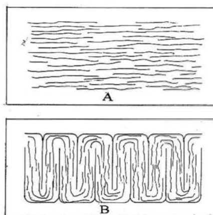
Figure 2. Typical positions of fibres in cross-laid (a) and perpendicular laid (b) textiles
