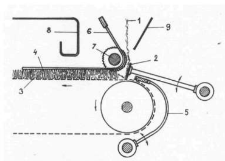
Figure 1. Perpendicular lapper
