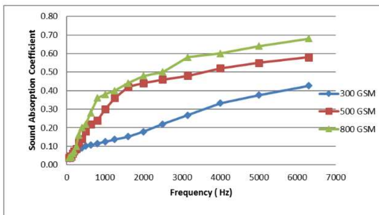
Figure 7. Sound absorption at various GSM levels
