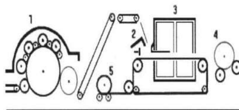
Figure 3. Production line for perpendicular laid textiles
