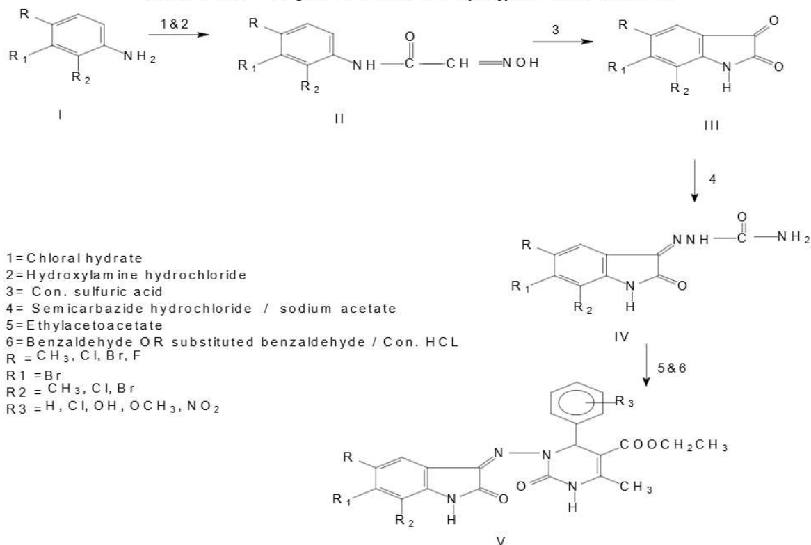
Scheme: 1: Schematic diagram of 3- substituted-[3,4-dihydro pyrimidinones]-Indolin-2-ones
