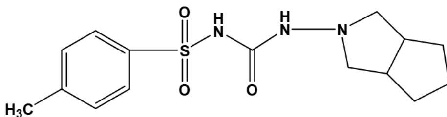
N-(hexahydrocyclopenta[c]pyrrol-2(1H)-ylcarbamoyl)-4-methylbenzenesulfonamide
