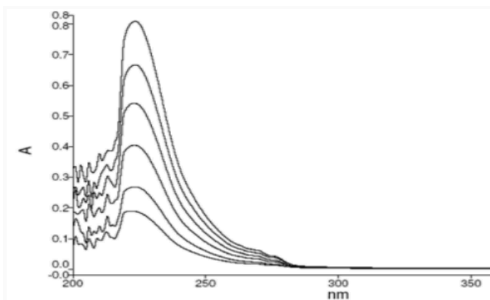
Figure 2: Zero order spectra of benzoylated product of PGL of 2.5\text{--}12.5\ \mu\text{g mL}^{-1} concentrations
